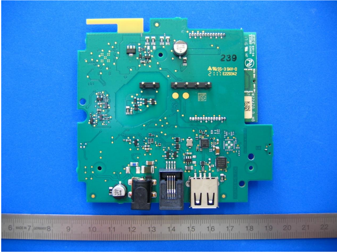
Photograph 4: Vitoconnect OT2 –Main PCB Bottom Side
