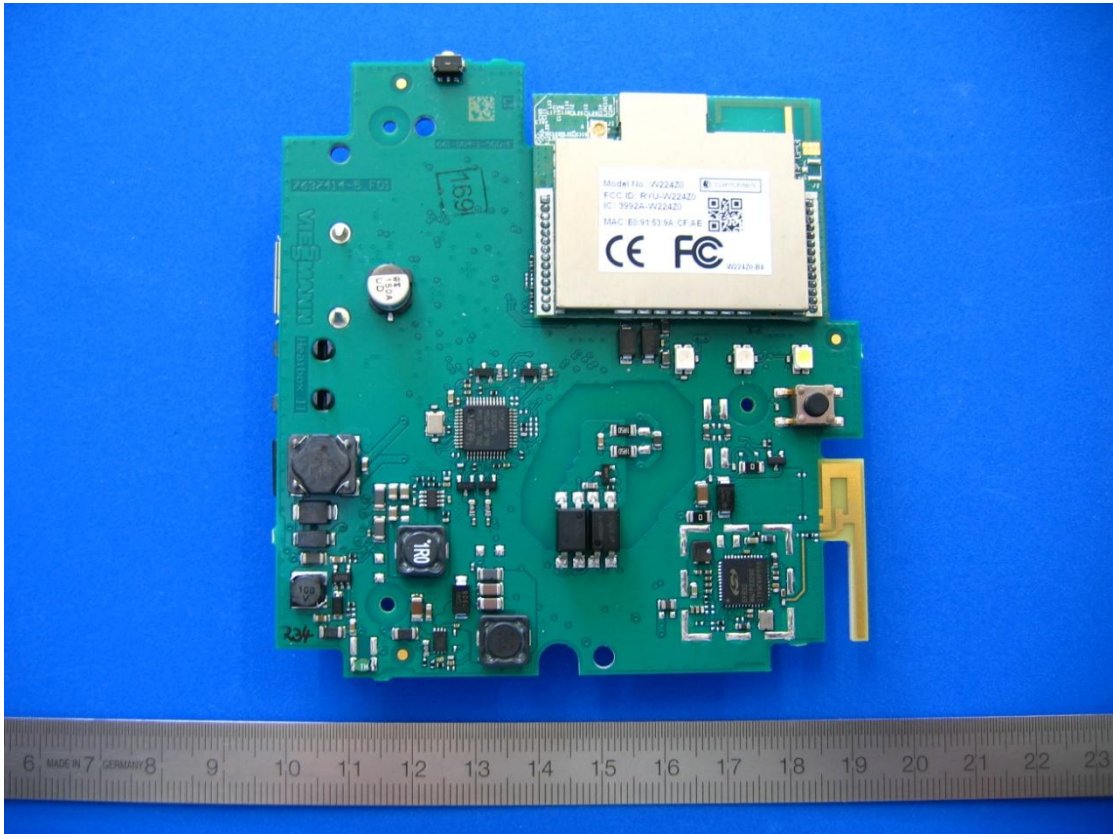
Photograph 3: Vitoconnect OT2 –Main PCB Top Side
