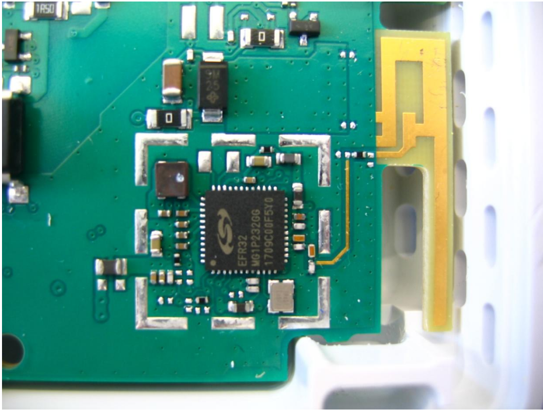
Photograph 7: ZigBee System-On-Chip and On-Board Antenna
