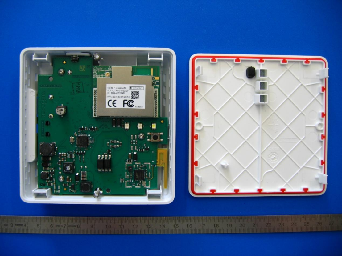
Photograph 2: Vitoconnect OT2 –Housing Top Side (inside)
