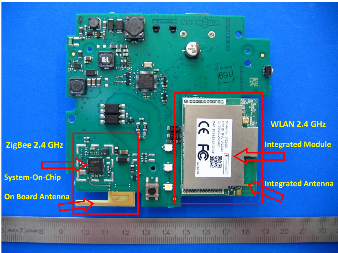
Photograph 5: Vitoconnect OT2 –Radio Modules + Onboard Antennas
