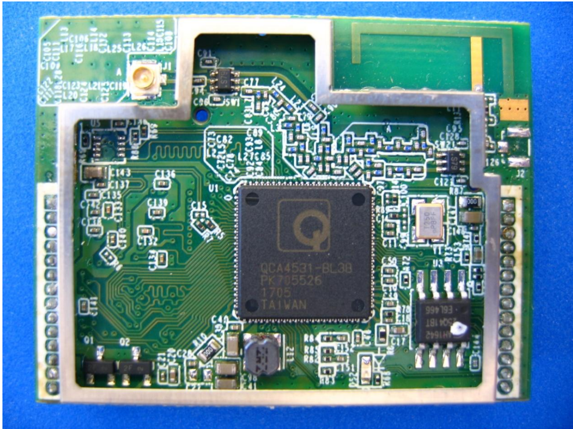
Photograph 6: WLAN Module without shielding plate
