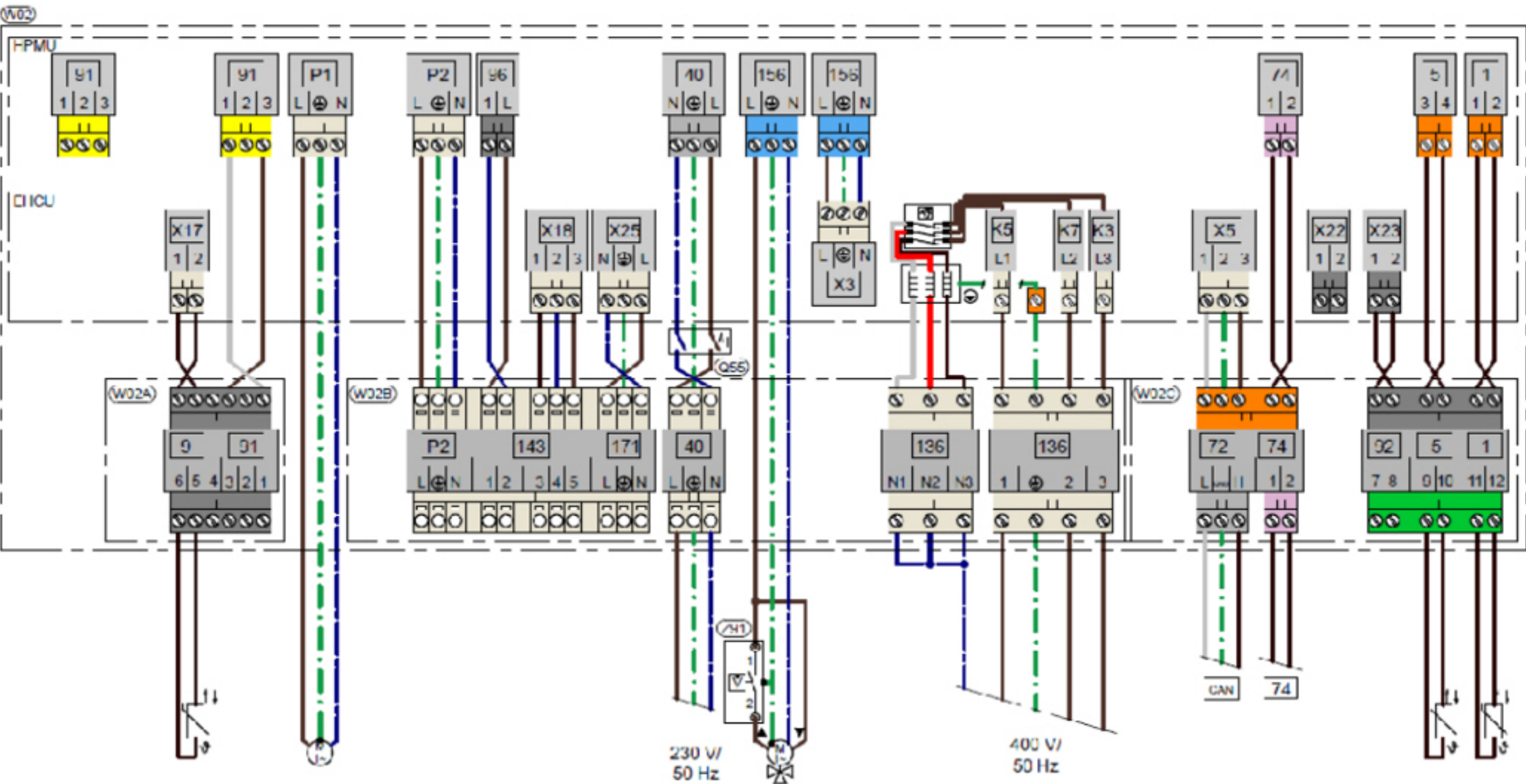
Schaltplan Original Viessmann
